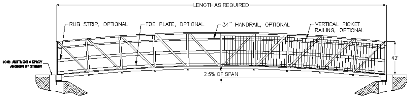
ELEVATION: TYPICAL CAMBERED BRIDGE
