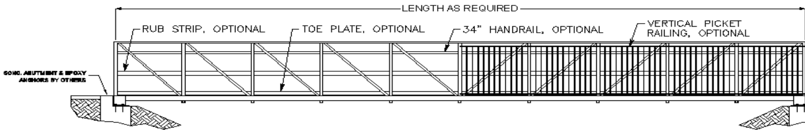
ELEVATION: TYPICAL FLAT BRIDGE
