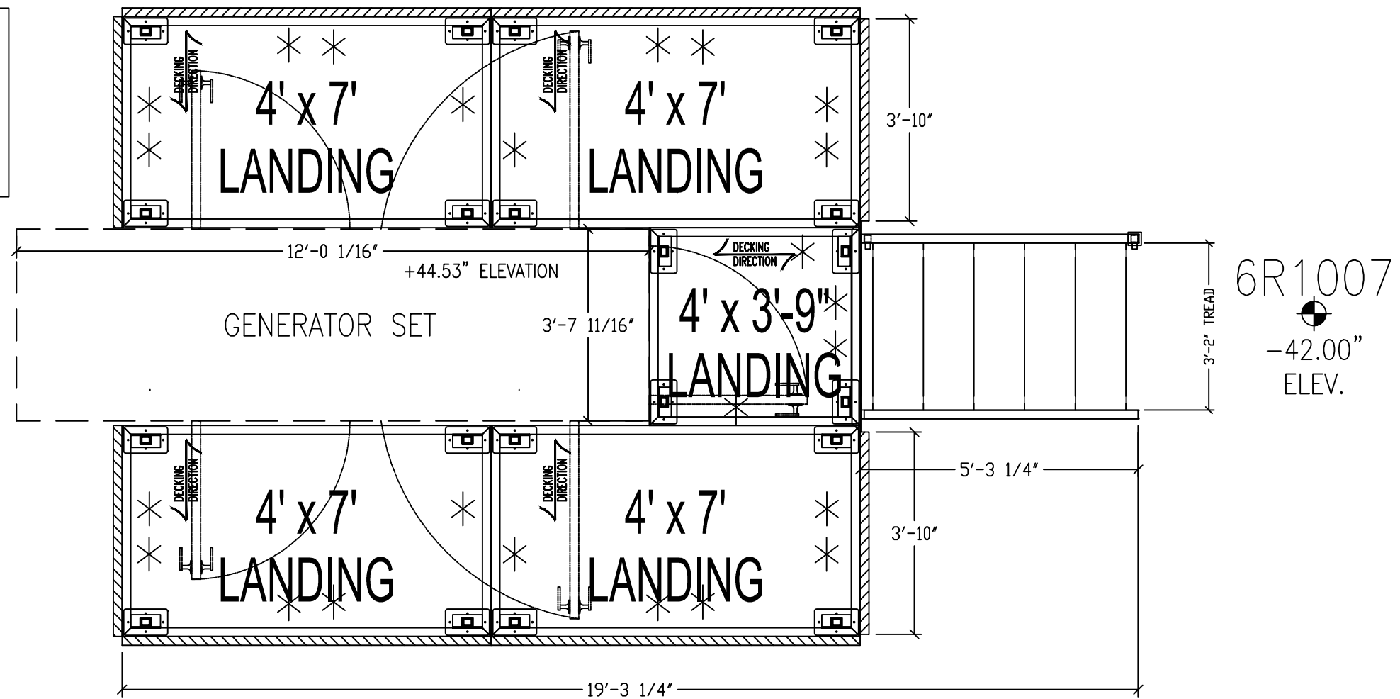
38 TWO LINE STAIR ACCESS PLAN VIEW
