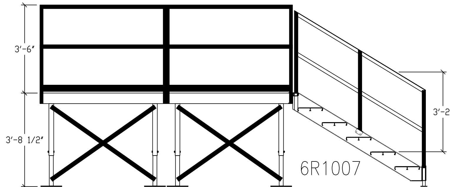
38 TWO LINE STAIR ACCESS ELEVATION VIEW
