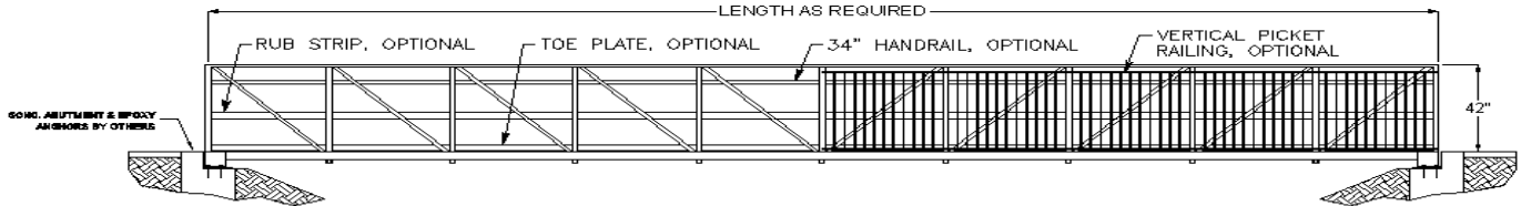
ELEVATION: TYPICAL FLAT BRIDGE
