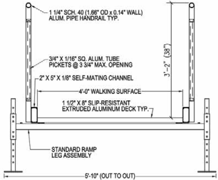
A-A 1 DETAIL 38 VP/TL RAMP CROSS SECTION SCALE: 3/4" = 1'-0"
