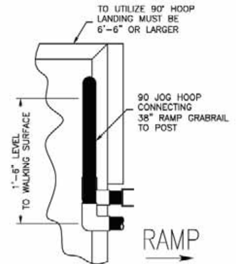
3 UPPER 90° HOOP DETAIL 2 38VP RAMP HANDRAIL (OPTIONAL)
