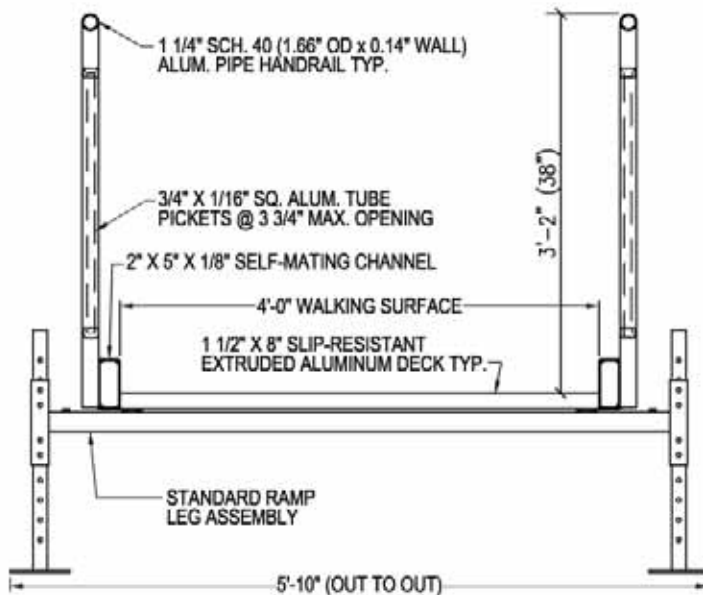
A-A 1 DETAIL 38" VP/TL RAMP CROSS SECTION SCALE: 3/4" = 1'-0"
