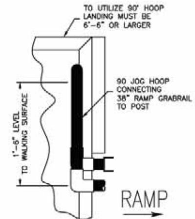
3 UPPER 90° HOOP DETAIL 2 38VP RAMP HANDRAIL (OPTIONAL)
