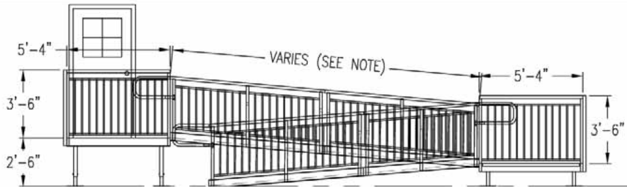
ELEV VIEW: 38 VP/TL ALUMINUM ACCESS RAMP SYSTEM NOTE: TO USE 38 VP/TL, MAX RUN OF RAMP SYSTEM=30'-0"
