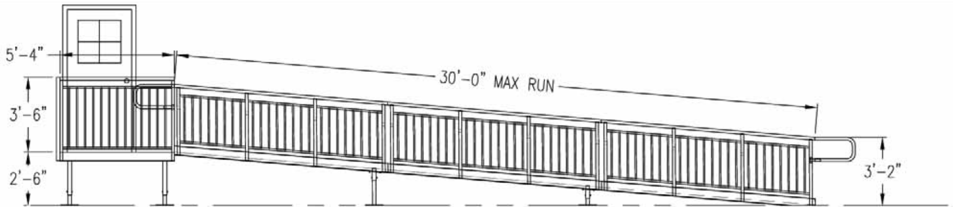
ELEVATION VIEW: 38 VP/TL ALUMINUM ACCESS RAMP SYSTEM
