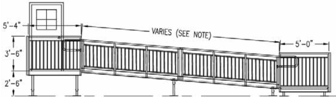
ELEV VIEW: 38 VP/TL ALUMINUM ACCESS RAMP SYSTEM NOTE: TO USE 38 VP/TL, MAX RUN OF RAMP SYSTEM=30'-0"
