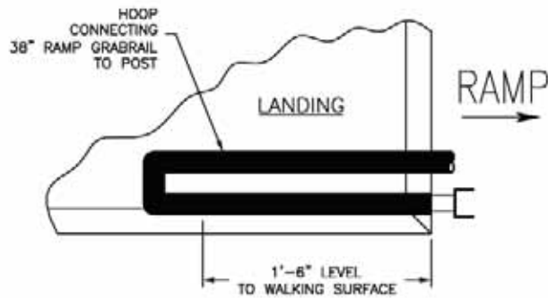
1 UPPER/LOWER HOOP DETAIL 2 38VP RAMP HANDRAIL
