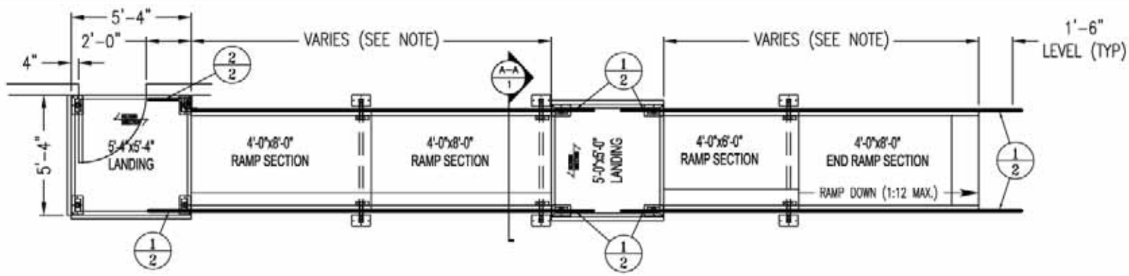
PLAN VIEW: 38 VP/TL ALUMINUM ACCESS RAMP SYSTEM
