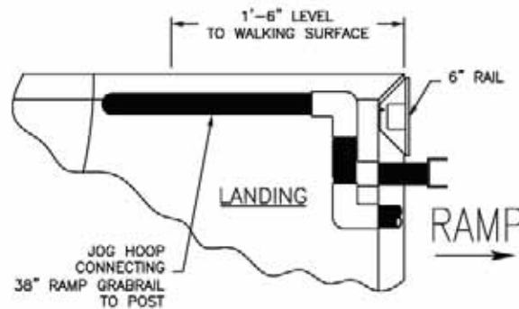
2 UPPER JOG HOOP DETAIL 2 38VP RAMP HANDRAIL
