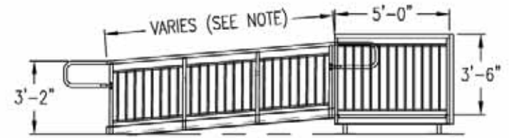
ELEV VIEW: 38 VP/TL ALUMINUM ACCESS RAMP SYSTEM NOTE: TO USE 38 VP/TL, MAX RUN OF RAMP SYSTEM=30'-0"
