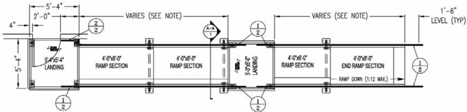
PLAN VIEW: 38 VP/TL ALUMINUM ACCESS RAMP SYSTEM
