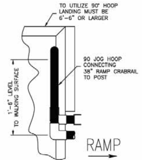
3 UPPER 90 degree HOOP DETAIL 2 38VP RAMP HANDRAIL (OPTIONAL)
